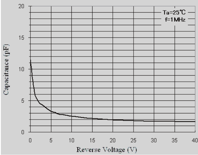
Fig.1 Total Capacitance
