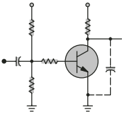
Figure 1. Switching Time Test Circuits
